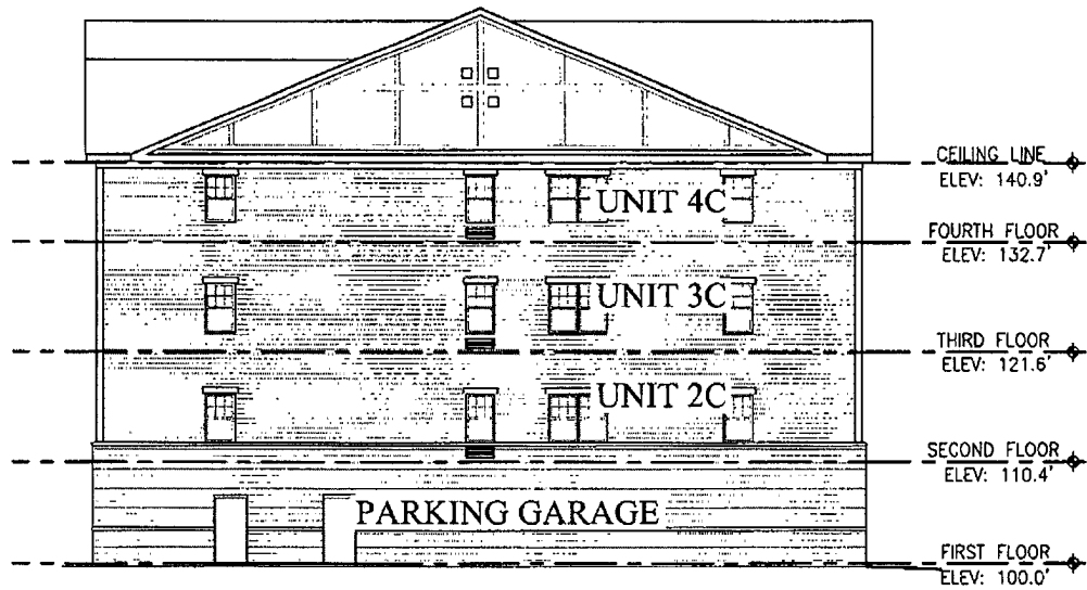
SOUTH ELEVATION
