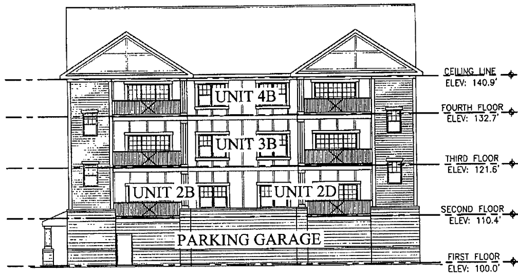
WEST ELEVATION
