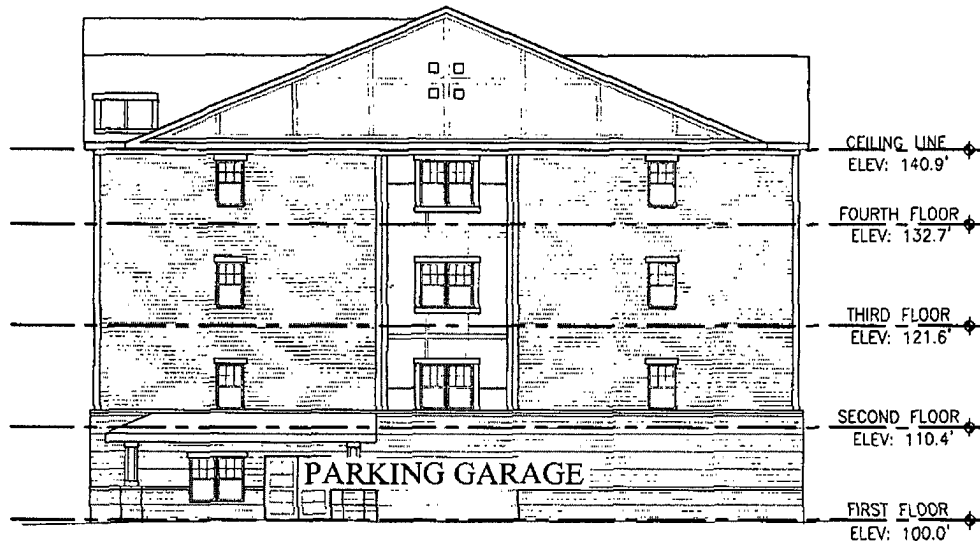
NORTH ELEVATION
